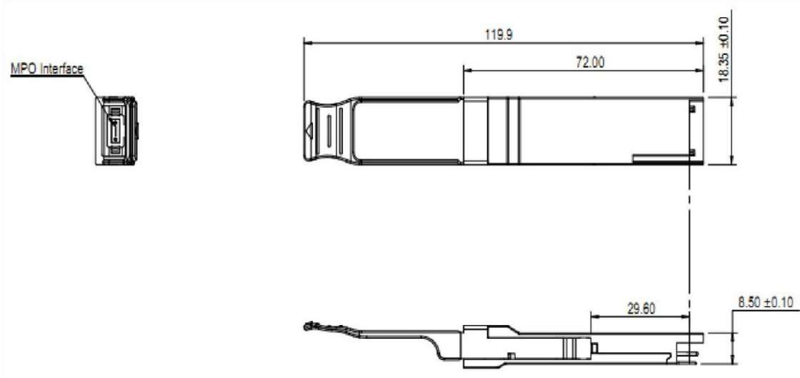
Figure 4 Package Dimensions
